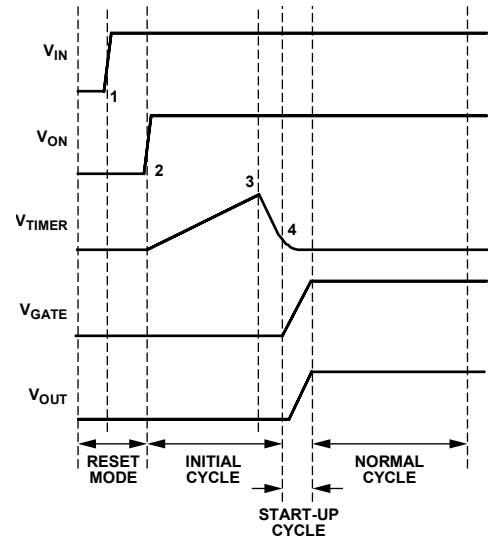
Figure 38. Power-Up Timing
