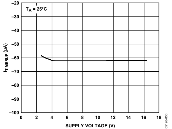
Figure 14. I_{TIMERUP} (During Cct Breaker Delay) vs. Supply Voltage
