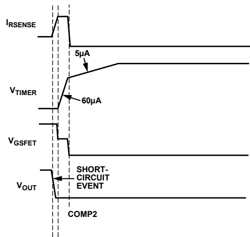
Figure 41. ADM1172-2 Latch Off After Overcurrent Fault
