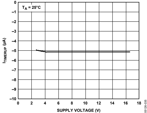
Figure 12. I_{TIMERUP} (In Initial Cycle) vs. Supply Voltage
