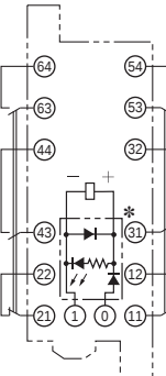
G7SA-3A3B Mounted
