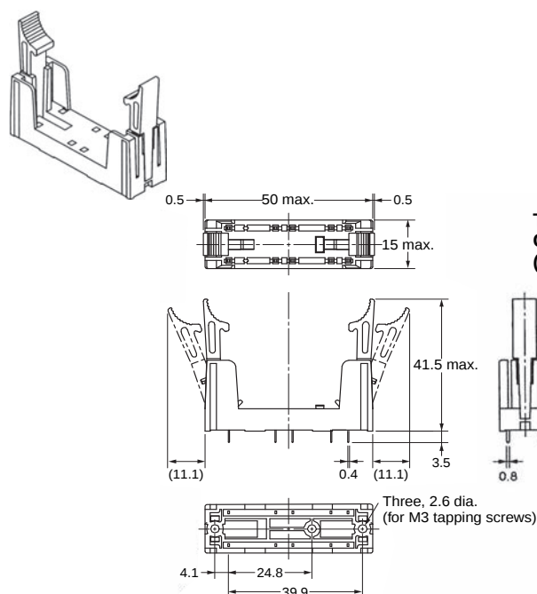
G7SA-3A1B Mounted
