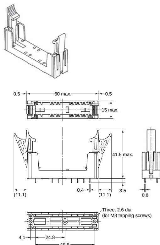
G7SA-5A1B Mounted
