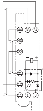
G7SA-2A2B Mounted
