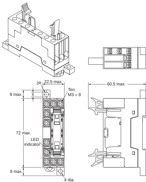
G7SA-3A1B Mounted
