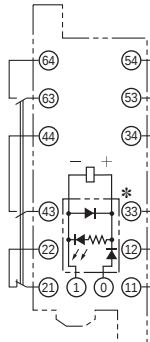
G7SA-4A2B Mounted
