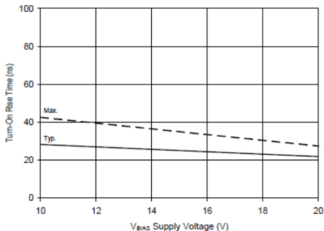
Figure 8B. Turn On Rise Time vs. Voltage
