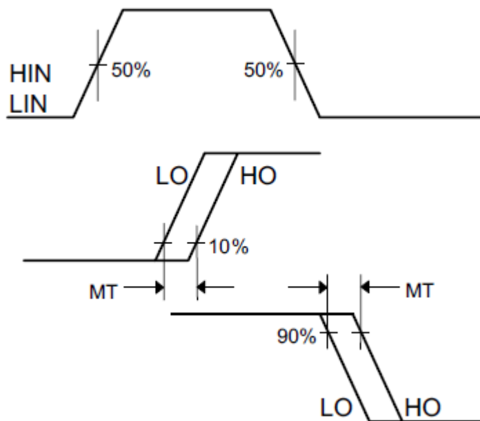
Figure 4. Delay matching Waveform Definitions
