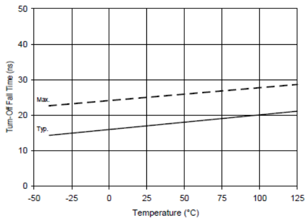
Figure 9A. Turn Off Fall Time vs. Temperature
