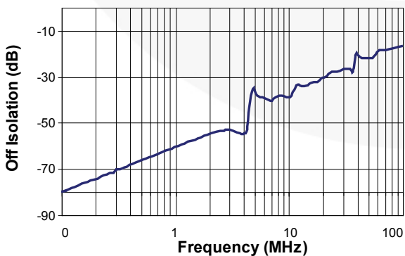
Figure 9. Frequency Response ( V_{CC}=5.0 V, C_L=0 pF)
