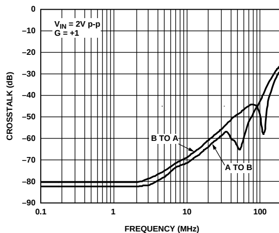
Figure 39. Crosstalk vs. Frequency (See Figure 51)
