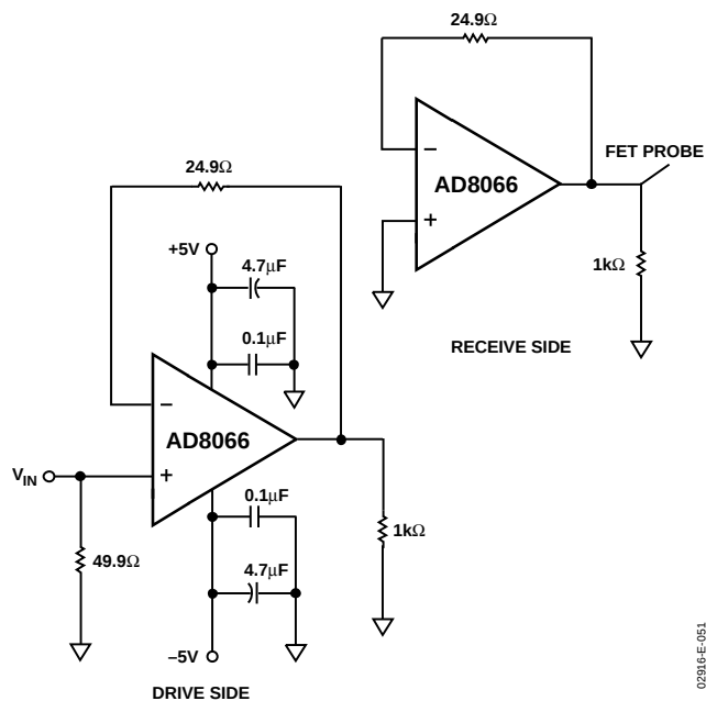
Figure 51. Crosstalk—AD8066
