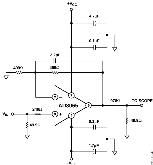
Figure 49. Settling Time
