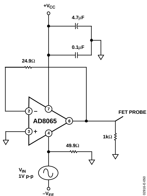
Figure 50. Negative PSRR
