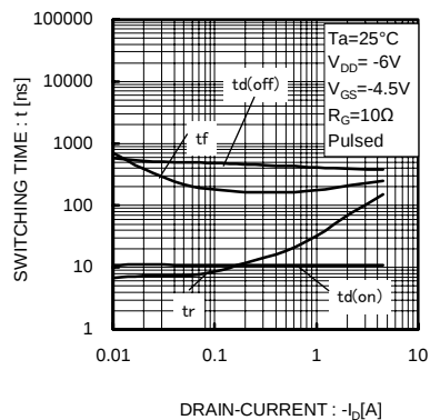
Fig.14 Switching Characteristics
