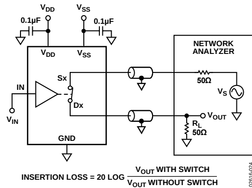
Figure 21. Bandwidth
