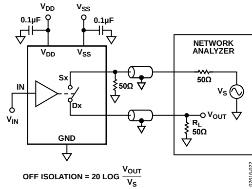
Figure 19. Off Isolation
