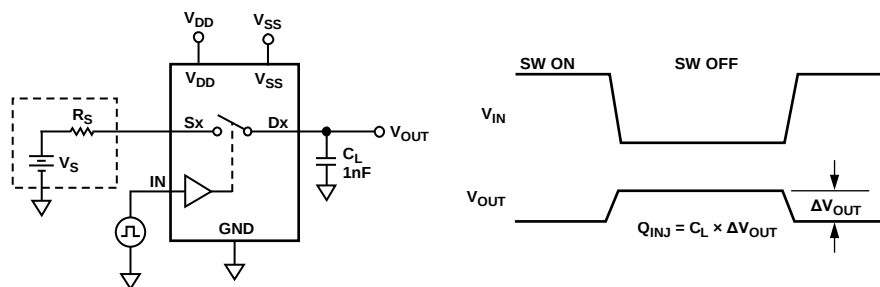
Figure 18. Charge Injection
