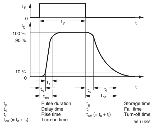
Fig. 3 - Switching Times
