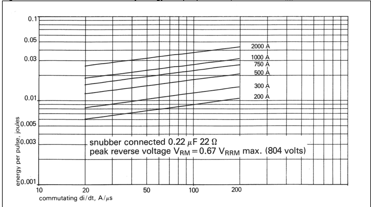
Figure 15 – Maximum reverse recovery energy loss per pulse at T_j = 125^\circ\text{C} and V_{rm} = 804 volts
