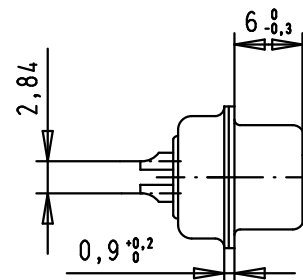
Solder bucket for AWG 20
