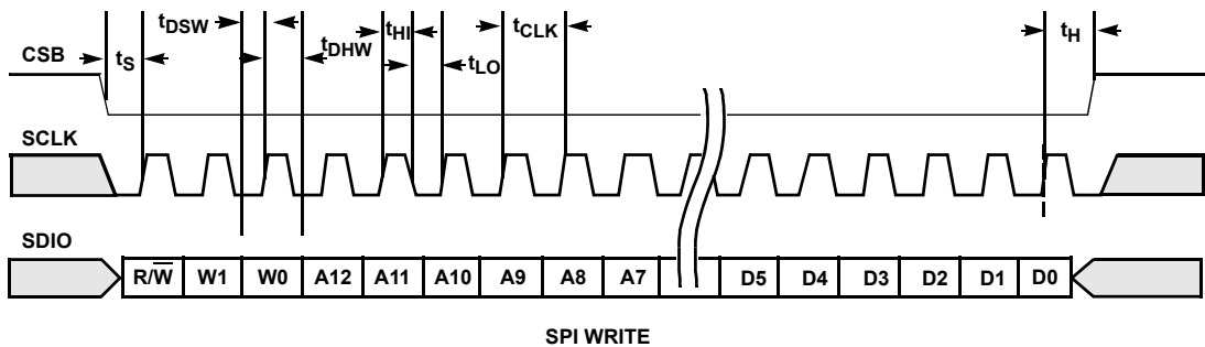
FIGURE 37. SPI WRITE
