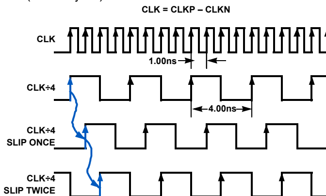
FIGURE 41. PHASE SLIP: CLK÷4 MODE, f_{\text{CLK}} = 1000\text{MHz}
