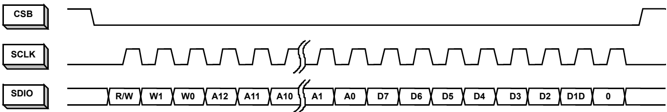
FIGURE 35. MSB-FIRST ADDRESSING
