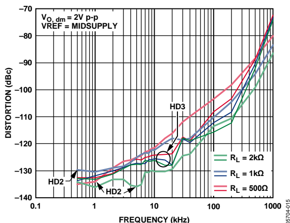
Figure 16. Distortion vs. Frequency for Various Loads
