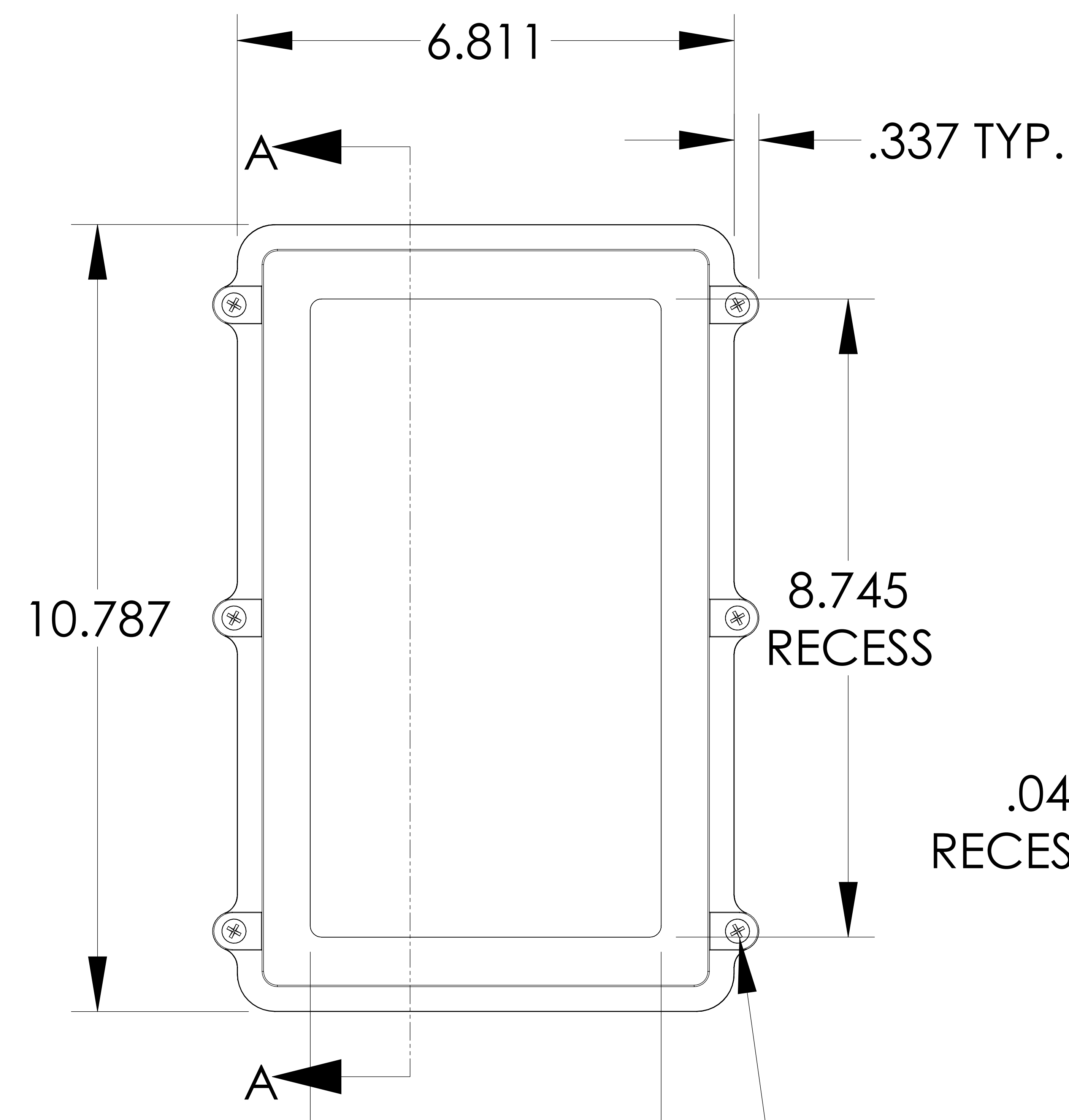
TOP VIEW
