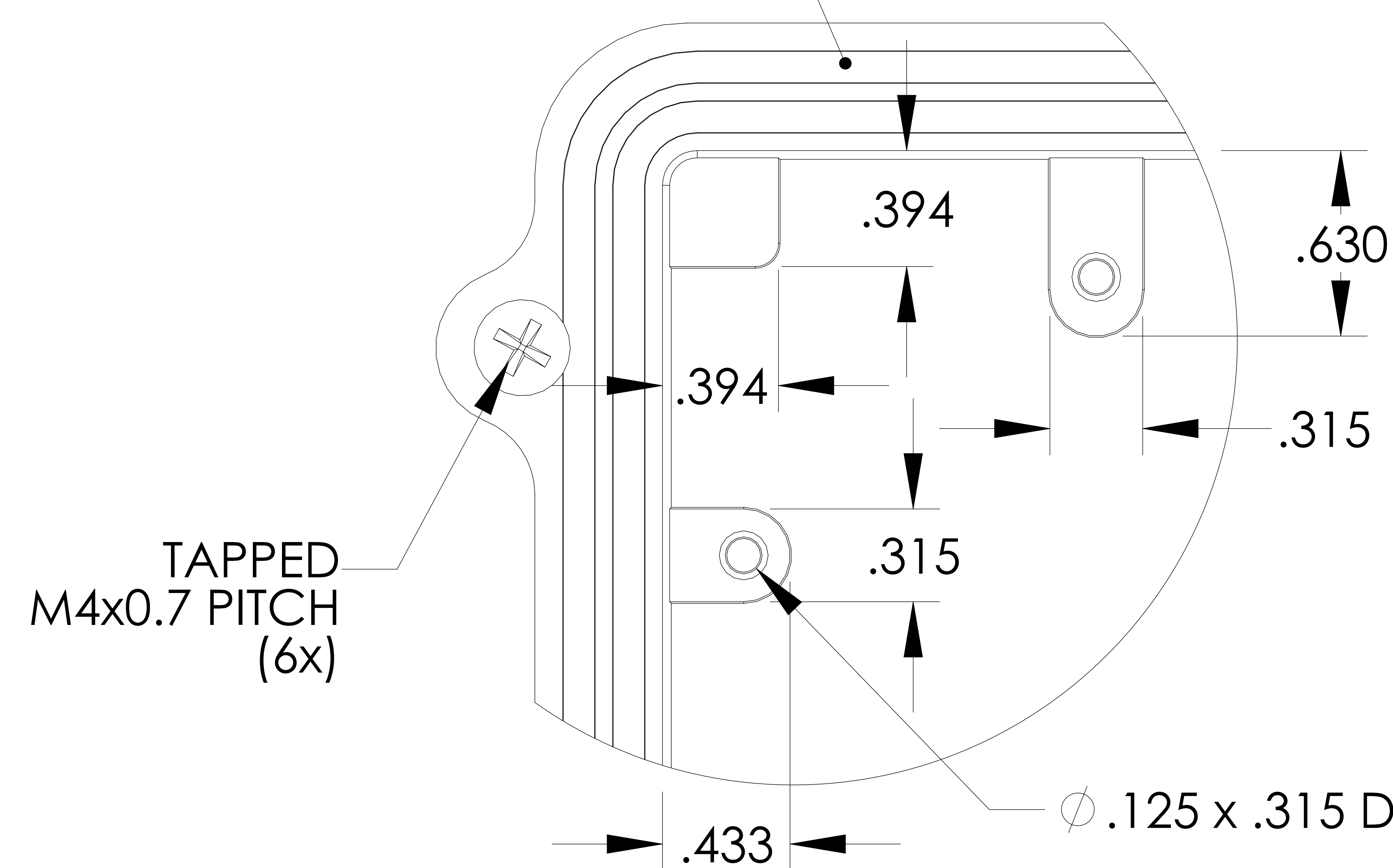
DETAIL B SCALE 4 : 1
