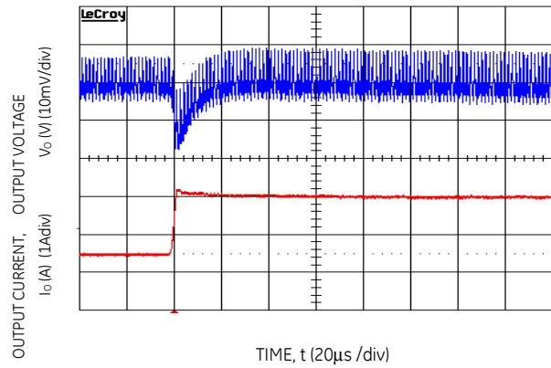
Figure 10. Transient Response to Dynamic Load Change from 50% to 100% at 12Vin, Cout-1x47uF+1x330uF, CTune-10nF & RTune-261
