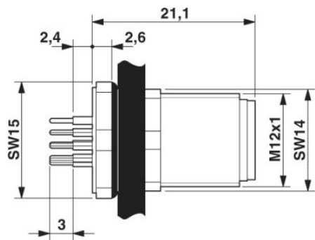
Dimensioned drawing
