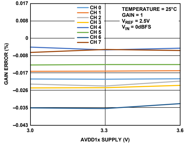
Figure 66. Gain Error vs. AVDD1x Supply, Low Power Mode
