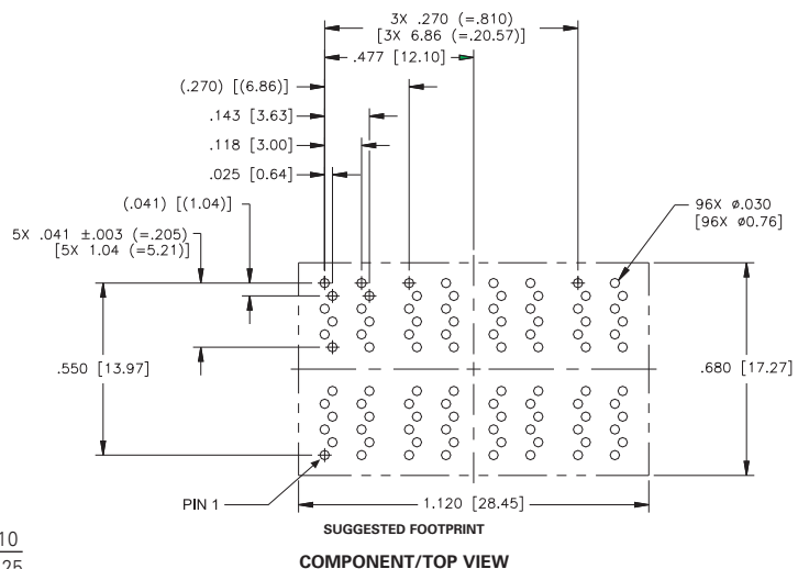
SUGGESTED FOOTPRINT COMPONENT/TOP VIEW
