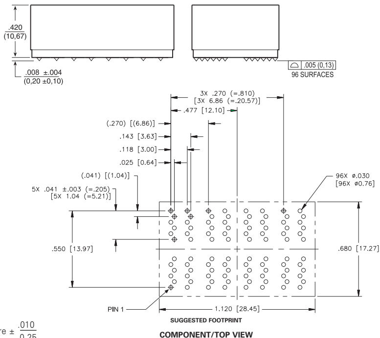
SUGGESTED FOOTPRINT COMPONENT/TOP VIEW
