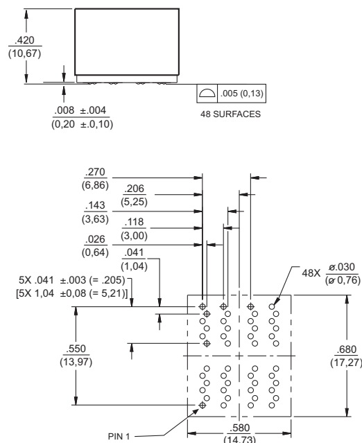
SUGGESTED FOOTPRINT COMPONENT/TOP VIEW
