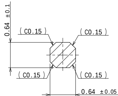
SECT. B-B (20 : 1)
