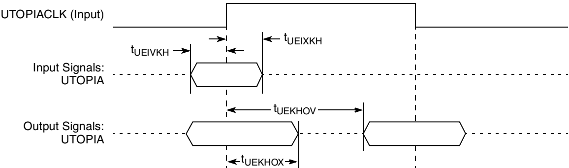
Figure 36. UTOPIA AC Timing (External Clock) Diagram
