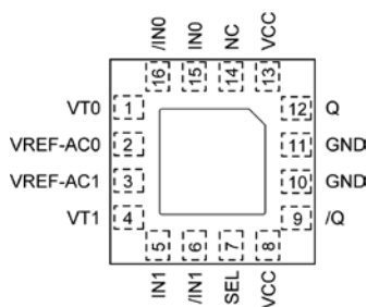
16-Pin QFN
