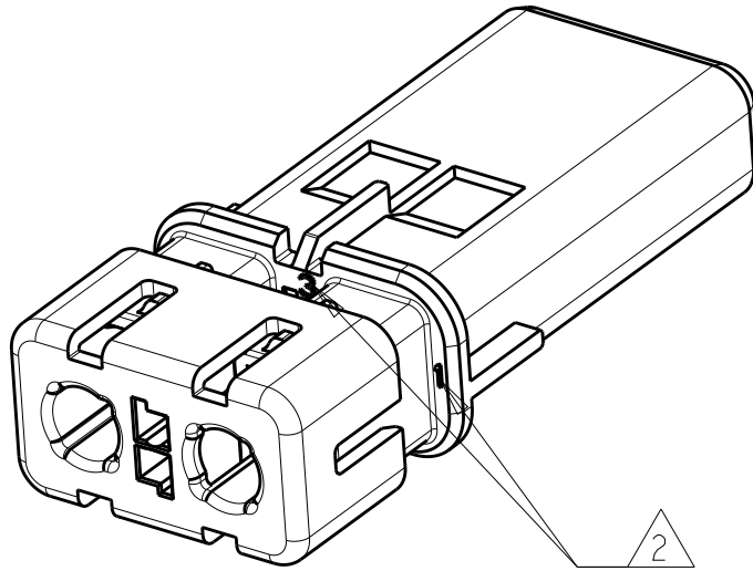
ISOMETRIC VIEWS SCALE 2:1
