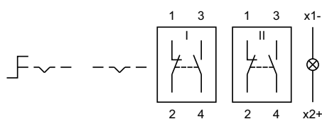
38 Selector switch 2 positions page 11 | Selector switch actuator 2 positions, flush mounting page 19
