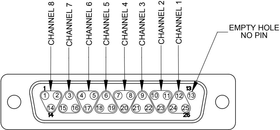
DB25 PIN-OUT VIEW FOR DB25
