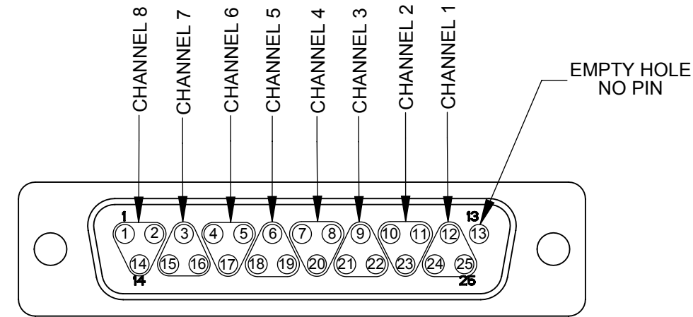
DB25 PIN-OUT VIEW FOR DB25
