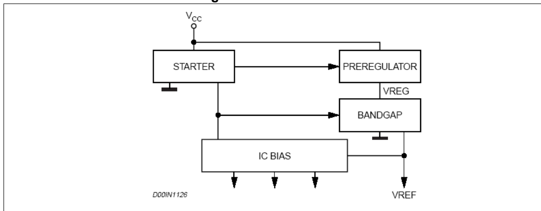
Figure 4. Internal circuit
