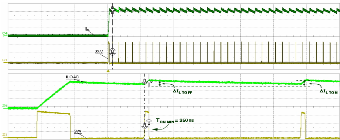
Figure 16. Short-circuit current V_{IN} = 24\text{ V}
