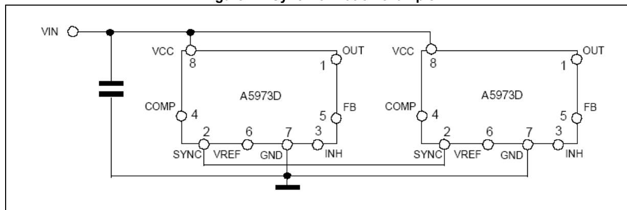
Figure 24. Synchronization example
