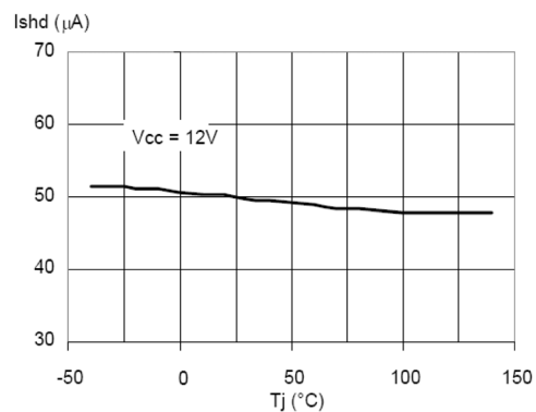
Figure 28. Shutdown current vs. junction temperature
