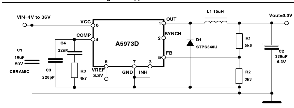
Figure 1. Application schematic
