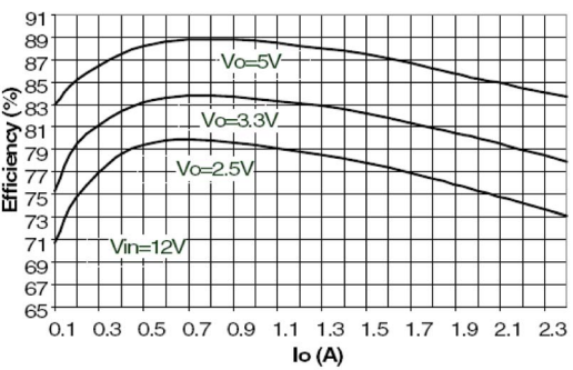
Figure 35. Efficiency vs. output current - V_{IN} = 12\text{ V}
