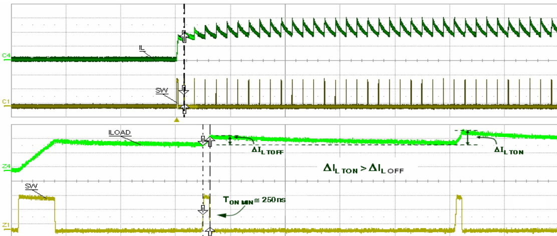
Figure 17. Short-circuit current V_{IN} = 36\text{ V}
