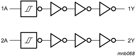
Figure 2. IEC logic symbol
