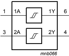
Figure 1. Logic symbol
