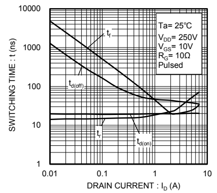
Fig.12 Switching Characteristics
