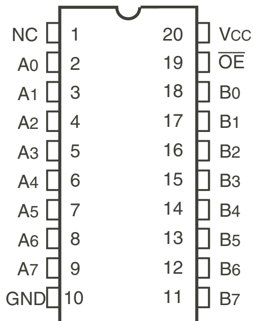
SOIC/ QSOP TOP VIEW
