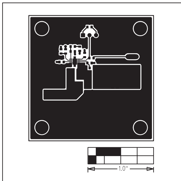
Figure 3. MAX17112 EV Kit PCB Layout—Component Side
