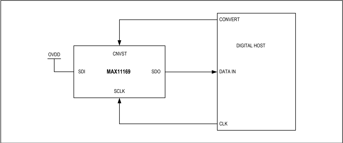
Figure 5. CS Mode 3-Wire, No-Busy Indicator Connection Diagram (SDI High)
