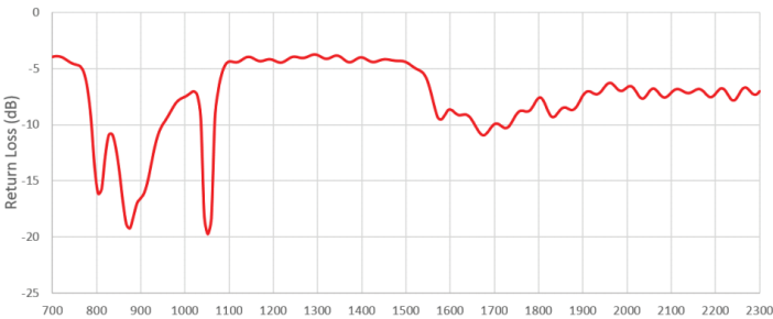
Return Loss
