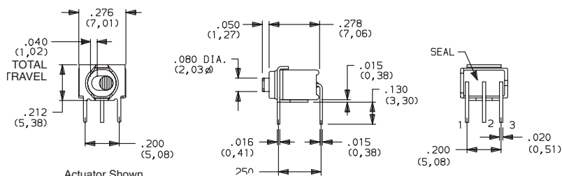
GS01MABE Horizontal Actuation SPDT
