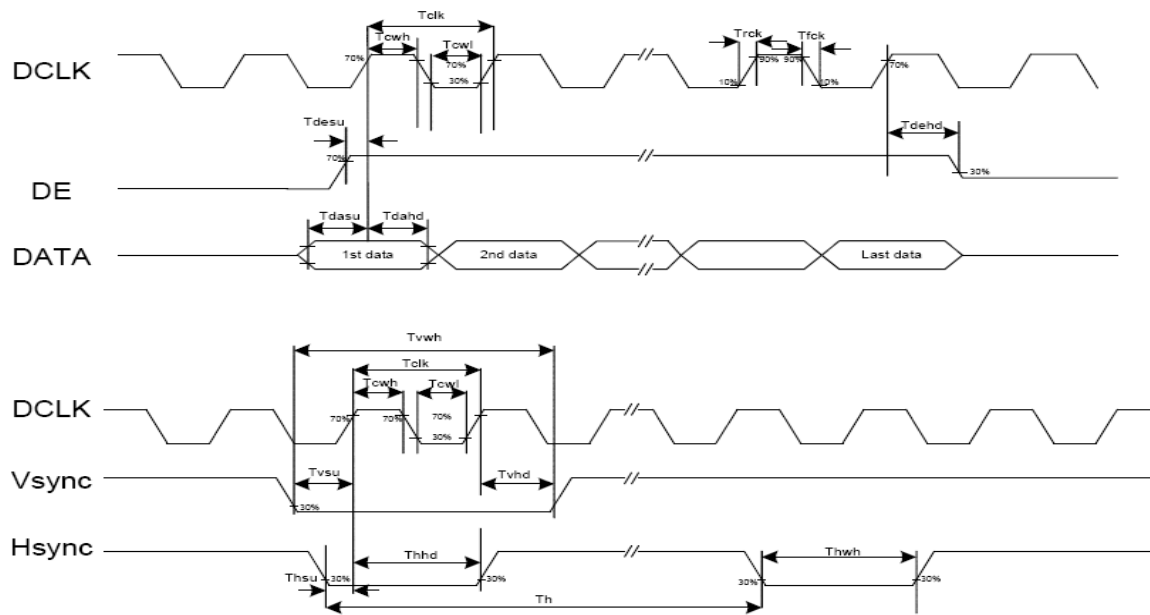
Figure 3: Pixel Timing
