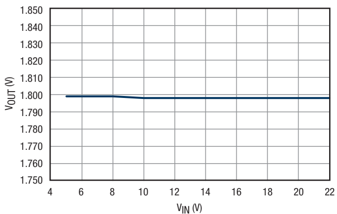
Figure 18. Line Regulation
