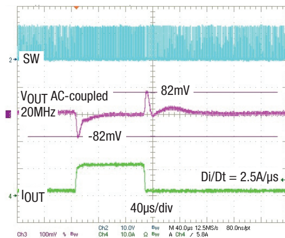
Figure 12. Load Transient, DCM, 1.8A-11.8A-1.8A
