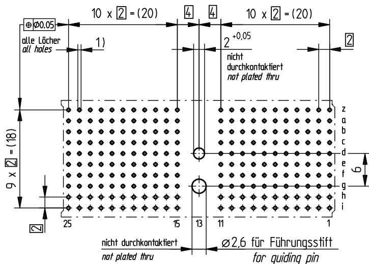
Board hole pattern (Component mounting side)
