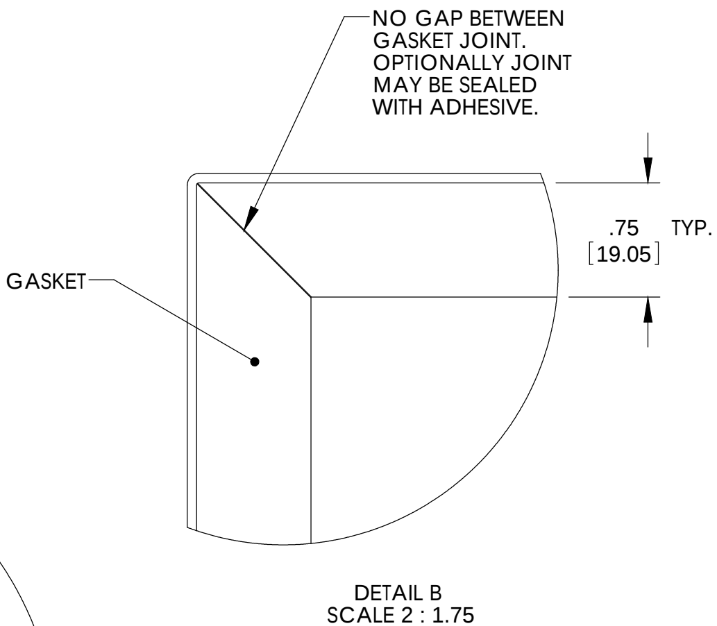
DETAIL B SCALE 2 : 1.75
