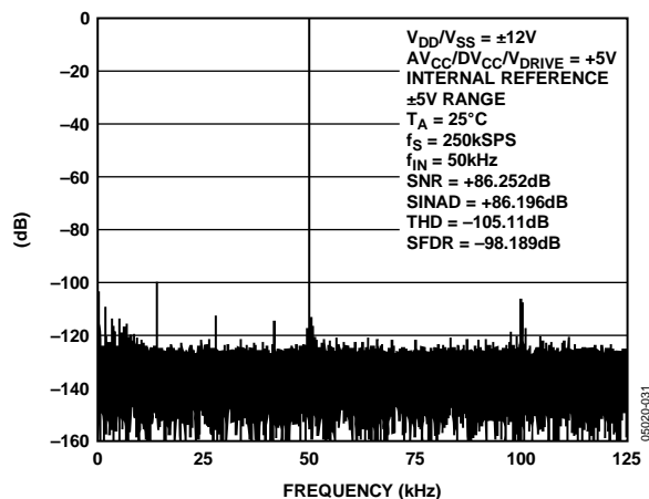
Figure 5. AD7656 FFT for \pm 5 V Range
