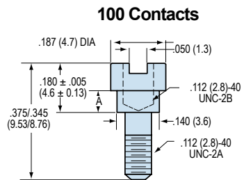
100 Contacts Kit Part Number 500-063-2 Kit Consists of Two Jackposts
