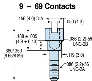
9 - 69 Contacts Kit Part Number 500-063-1 Kit Consists of Two Jackposts
