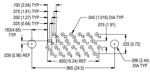
25 PIN MWDM-25PCBS
