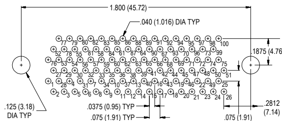
100 Socket MWDM-100SCBS
