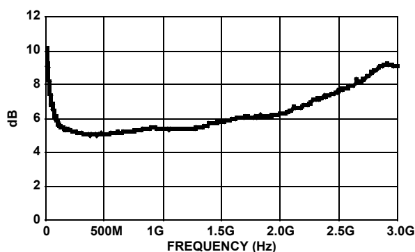
FIGURE 27. NOISE FIGURE vs FREQUENCY
