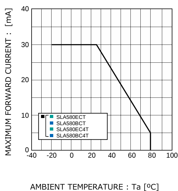
Fig.4 Derating
