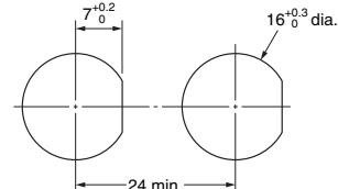
Panel Cutouts
