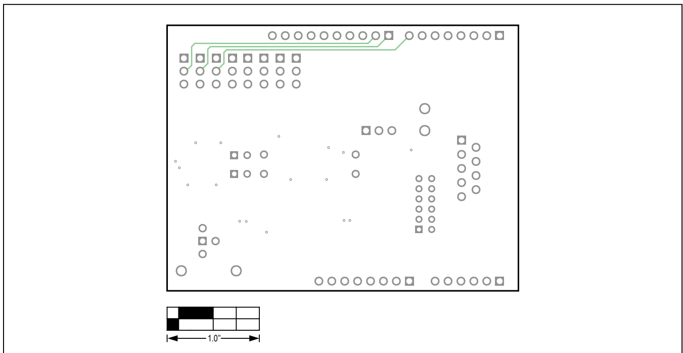
MAX33251E Shield—Internal Layer 3
