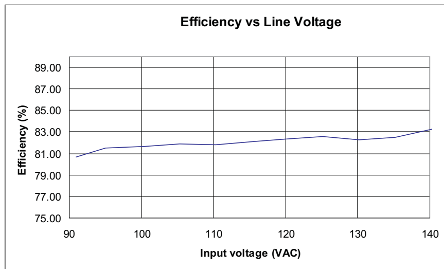
Figure 3. LM3447-A19-120VEVM Efficiency
