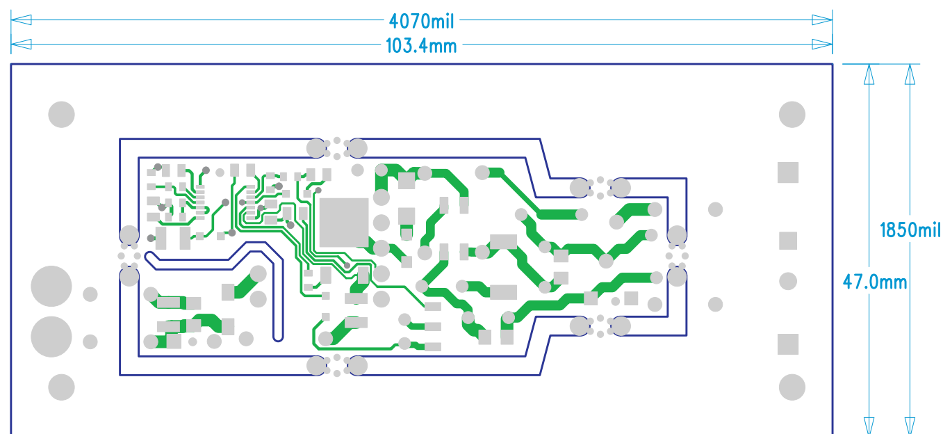
Figure 30. LM3447-A19-120VEVM Bottom Layer Copper (bottom view)
