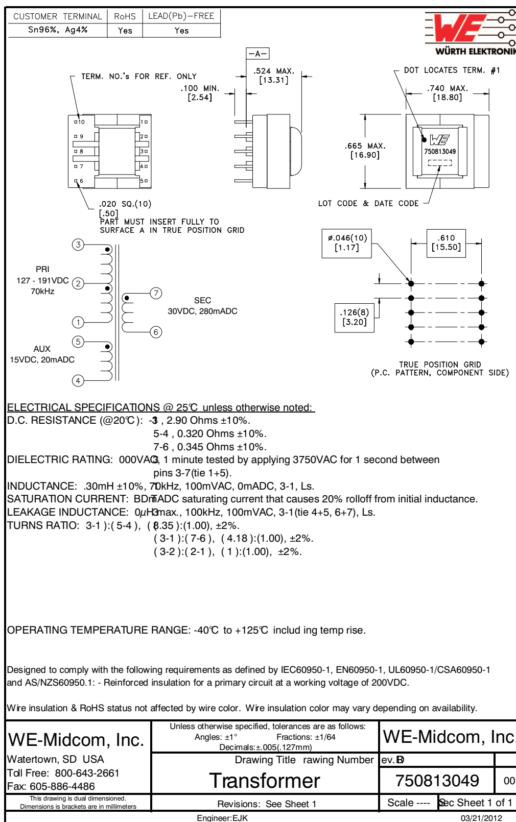
Figure 28. Transformer Specification
