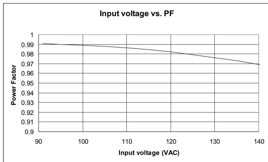
Figure 4. LM3447-A19-120VEVM Power Factor vs Line Voltage
