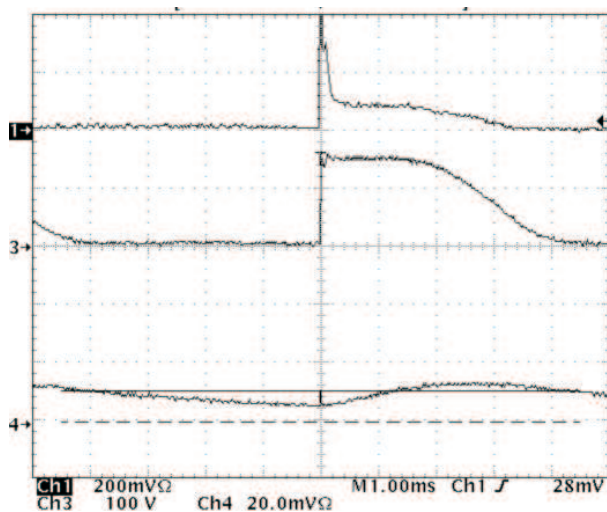
Figure 17. Dimmer 4 ms (Ch4- LED current Ch3 - rectified line voltage Ch1 – line current)
