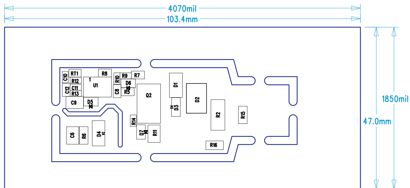
Figure 32. LM3447-A19-120VEVM Bottom Assembly Drawing (bottom view)
