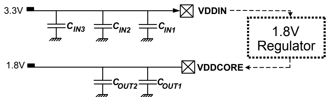
Figure 6-1. Supply Decoupling
