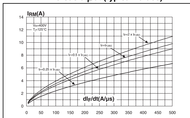
Figure 5. Peak reverse recovery current versus dl_F/dt (typical values)
