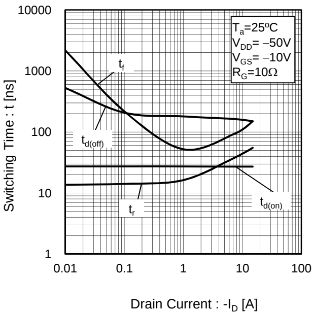
Fig.20 Switching Characteristics
